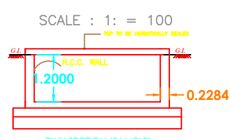
RW_SECTION (SAMPLE) RW_CAPACITY_L = 2000LTRS
