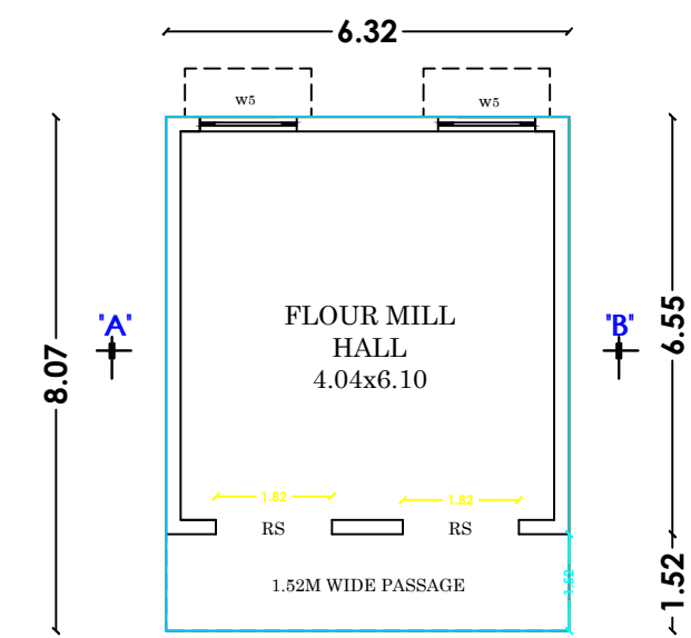
FLOOR 0 GROUND FLOOR PLAN
