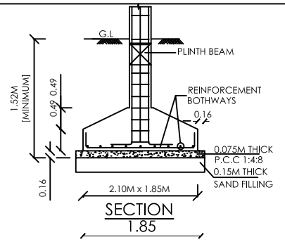
SECTION 1.85
