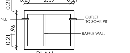
PLAN SEPTIC. TANK
