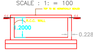
RWH_SECTION (SAMPLE)
