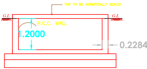
RWH SECTION (SAMPLE)
