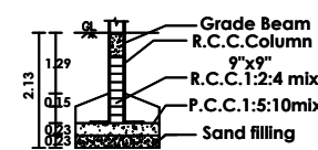
COLUMN DETAILS
