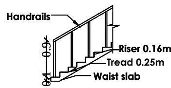
STAIRCASE DETAILS
