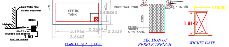
PLAN OF SEPTIC TANK
