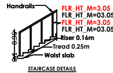
STAIRCASE DETAILS
