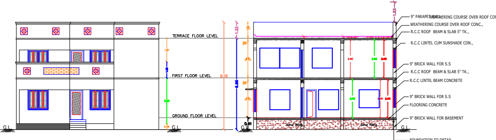
FRONT ELEVATION
