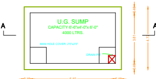
U.G. SUMP CAPACITY 6'0" X 4'0" X 6'0" 4000 LTRS. NEW HOLE COVER 22" DIA. DRAIN 1 1/2"
