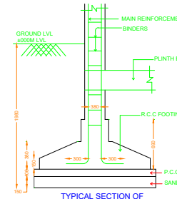
TYPICAL SECTION OF R.C.C. COLUMN FOUNDATION SCALE : 1" = 2'-0"
