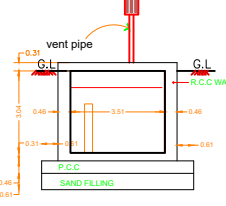
SECTION ON D-D
