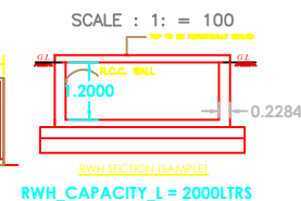
RWL SECTION (SAMPLE)
