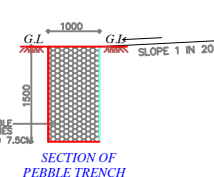
SECTION OF PEBBLE TRENCH
