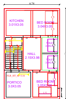
PROPOSED GROUND FLOOR PLAN
