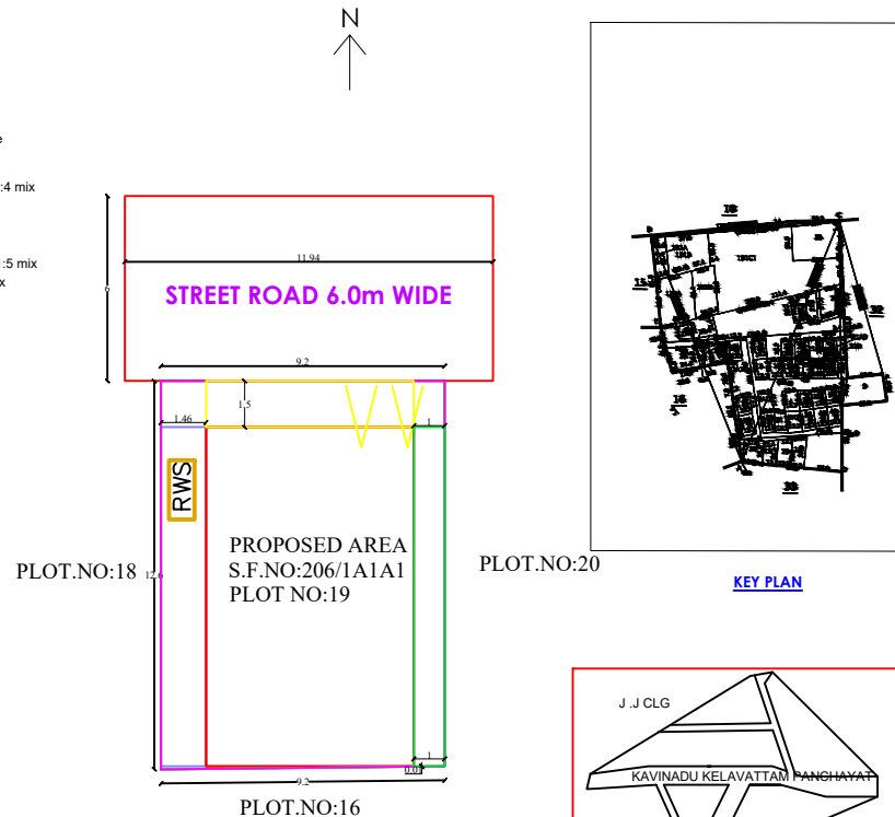
SITE PLAN-SCALE1:100
