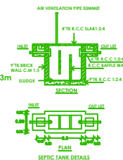
SEPTIC TANK DETAIL
