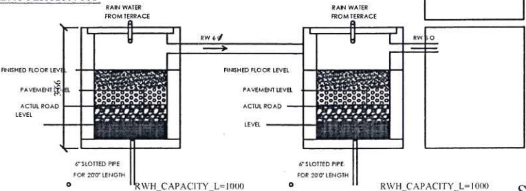
RAIN WATER PERCOLATION PIT
