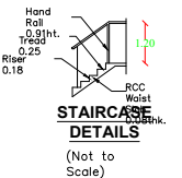
STAIRCASE DETAILS (Not to Scale)
