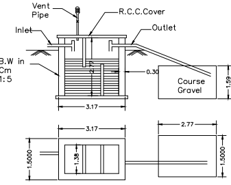
SEPTIC TANK & D-TRENCH DETAILS
