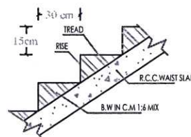
SECTION OF STAIRCASE
