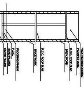
SECTION ON XX
