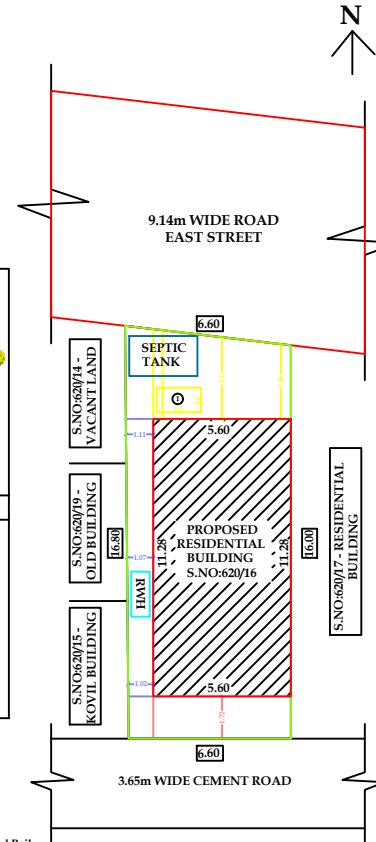
SITE PLAN SCALE:1:100
