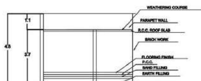
SECTION ON AA
