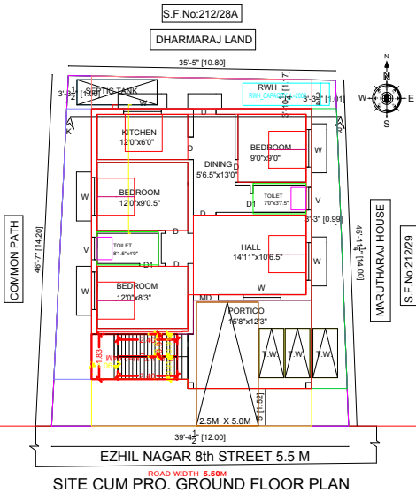
SITE CUM PRO. GROUND FLOOR PLAN
