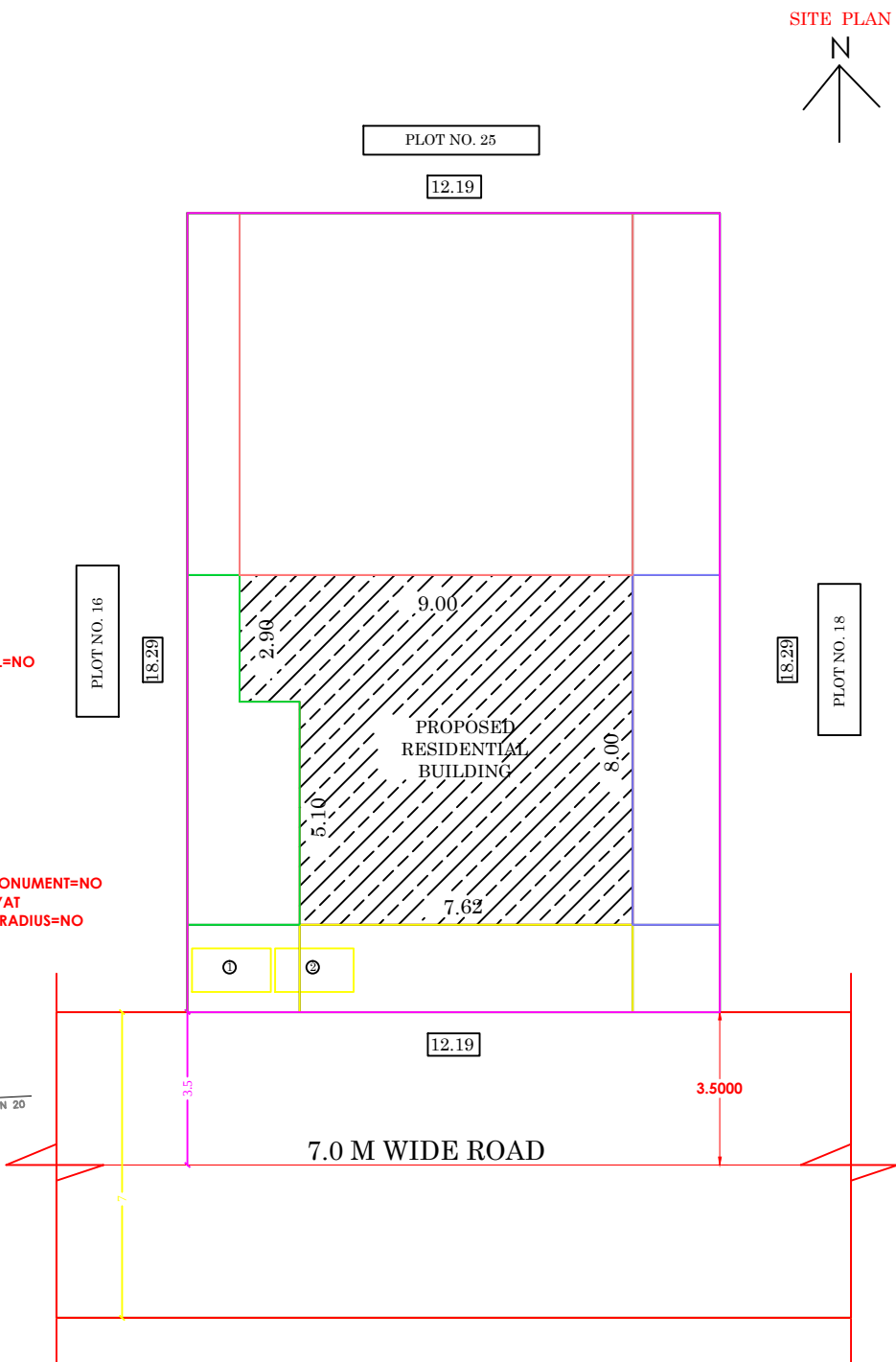
SITE PLAN
