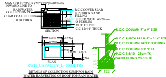
COLUMN DETAILS
