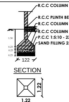
COLUMN DETAILS PLAN
