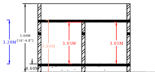
SECTION ON XX
