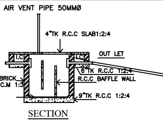
SECTION
