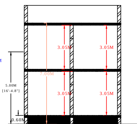
SECTION ON XX
