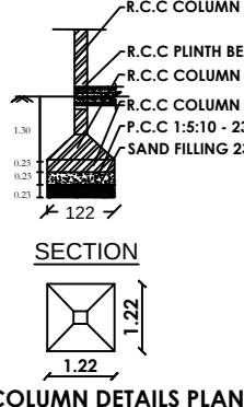
COLUMN DETAILS PLAN
