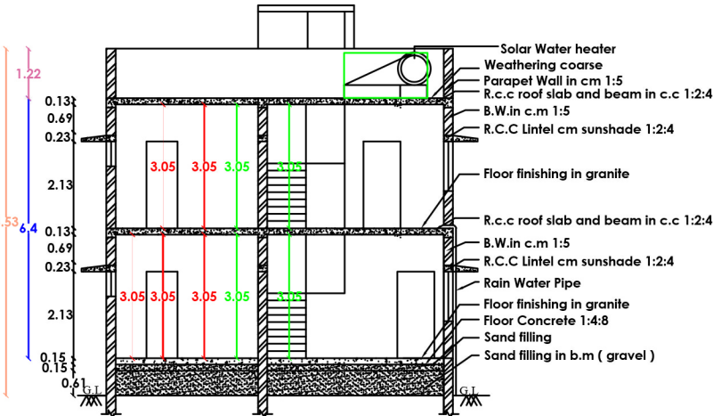
SECTION - "AB,CD"
