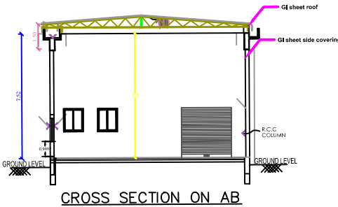
CROSS SECTION ON AB
