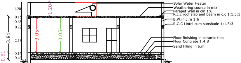
SECTION - "AB "
