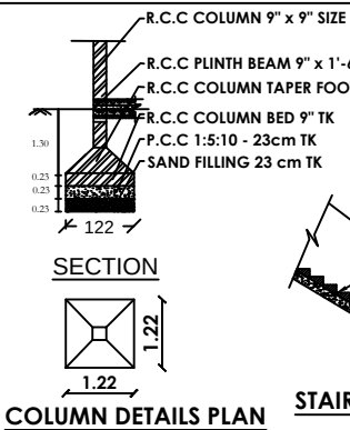
COLUMN DETAILS PLAN
