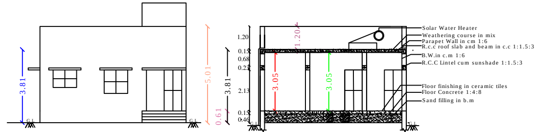
SECTION - "AB "
