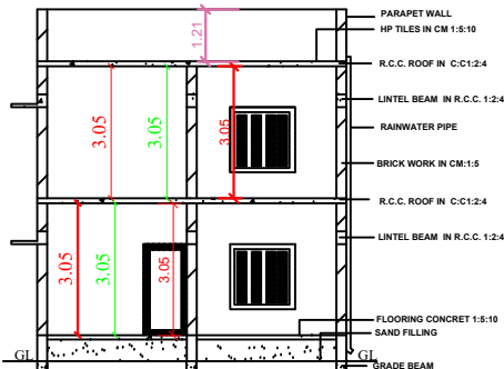
CROSS SECTION ON "A & A"
