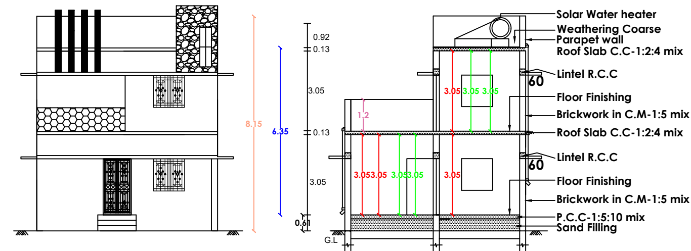
ELEVATION SECTION "AB"
