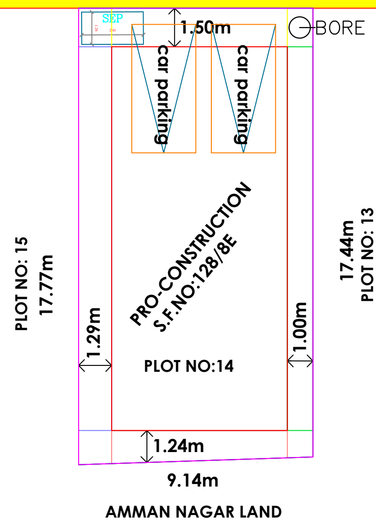
SITE PLAN-SCALE1:100
