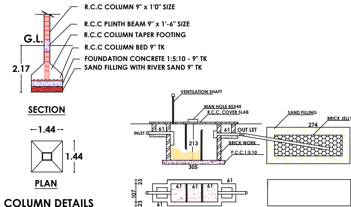
COLUMN DETAILS
