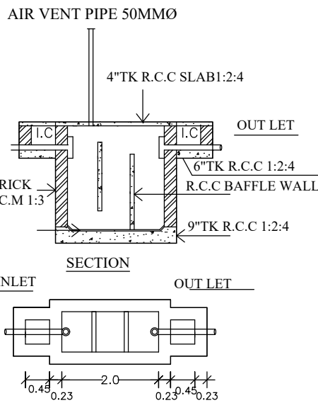
PLAN SEPTIC TANK DETAILS
