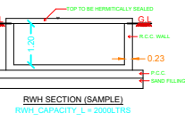
RWVH SECTION (SAMPLE) RWVH_CAPACITY_1 = 2000 LTRS
