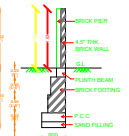
COMPOUND WALL DETAIL
