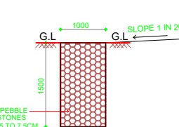
SECTION OF PEBBLE TRENCH SCALE : 1 : = 100
