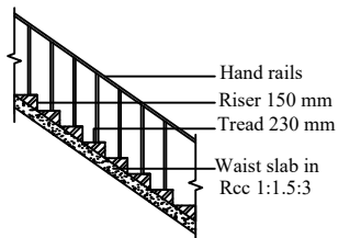
DETAILS OF STAIR CASE
