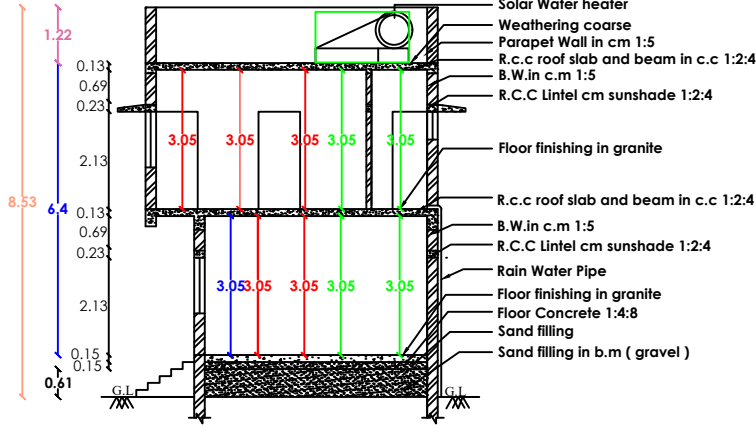
SECTION - "AB,CD"
