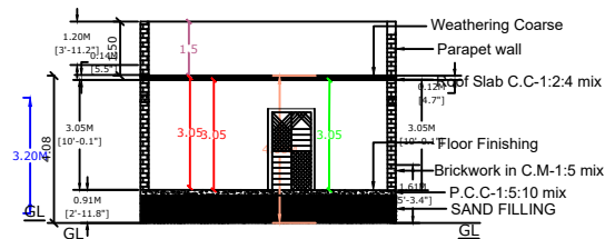
CROSS SECTION ON AB
