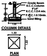
COLUMN DETAILS
