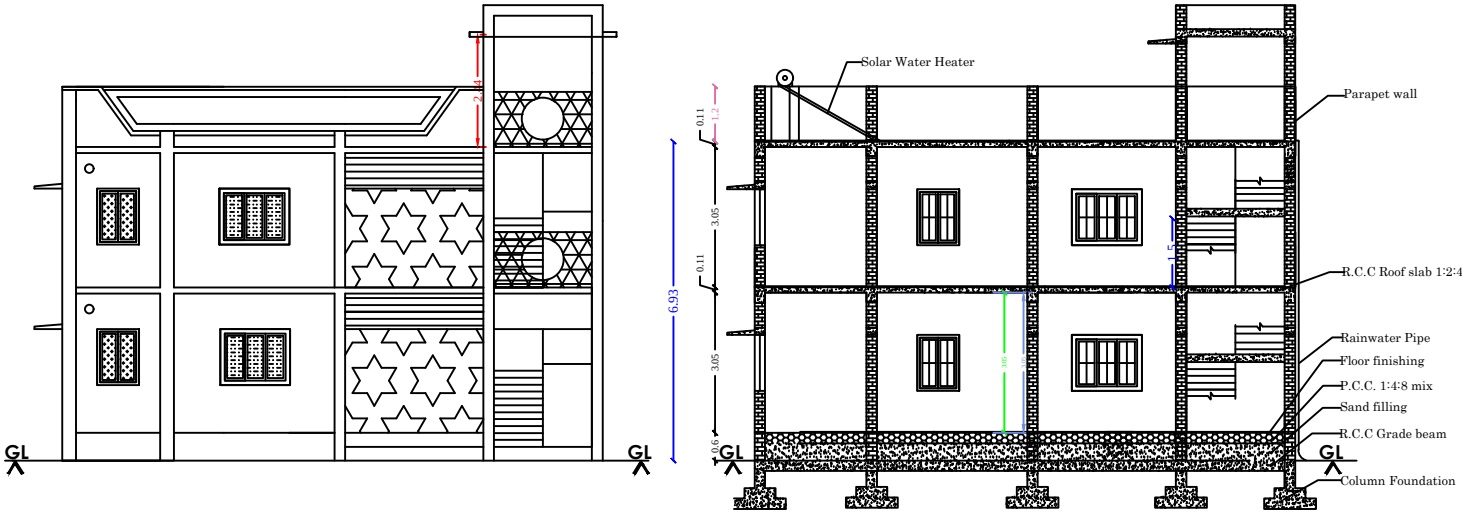
FRONT ELEVATION
