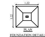
FOUNDATION DETAILS
