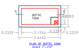
PLAN OF SEPTIC TANK
