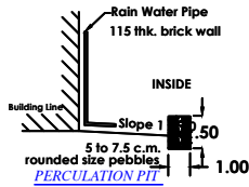
PERCUSSION PIT
