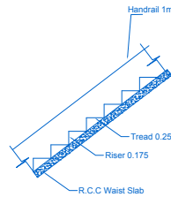
STAIR DETAILS
