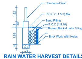
RAIN WATER HARVEST DETAILS
