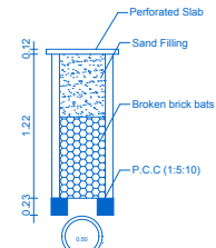
RAIN WATER COLLECTION WELL
