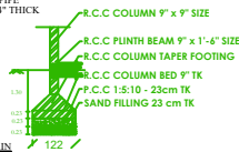
COLUMN DETAILS PLAN STAIRCASE DETAILS
