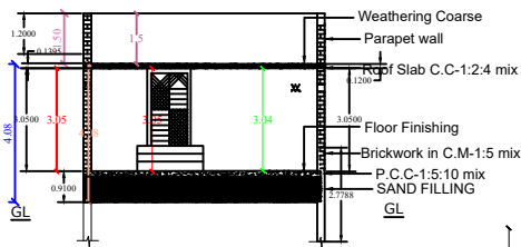
CROSS SECTION ON AB
