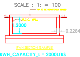
RWH_CAPACITY_L = 2000LTRS
