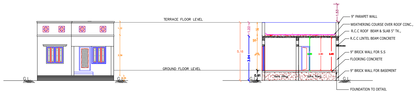
FRONT ELEVATION
