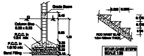
COLUMN DETAILS NOT TO SCALE
