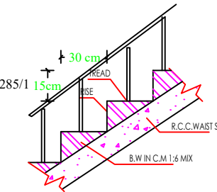
SECTION OF STAIRCASE
