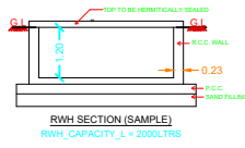
RWH SECTION (SAMPLE) NOT TO SCALE
