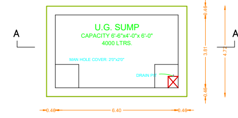
SUMP DETAIL SCALE 1"=4'0"
