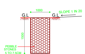
SECTION OF PEBBLE TRENCH SCALE : 1: = 100
