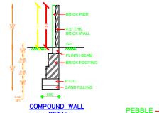
COMPOUND WALL DETAIL NOT TO SCALE
