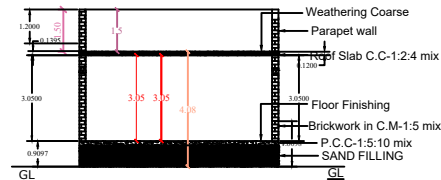
CROSS SECTION ON AB
