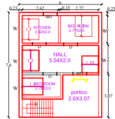
PROPOSED GROUND FLOOR PLAN
