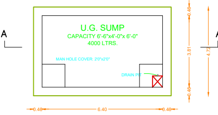
SUMP DETAIL
