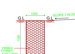
SECTION OF PEBBLE TRENCH
