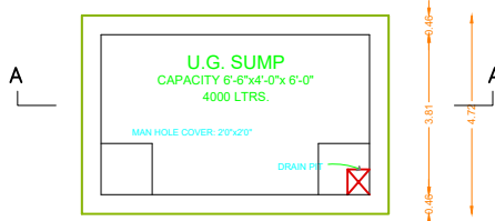
SUMP DETAIL
