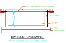
RWI SECTION (SAMPLE)
