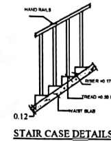
STAIR CASE DETAILS
