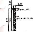
DETAILS OF PERCOLATION PIT
