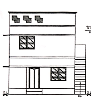
Front Elevation
