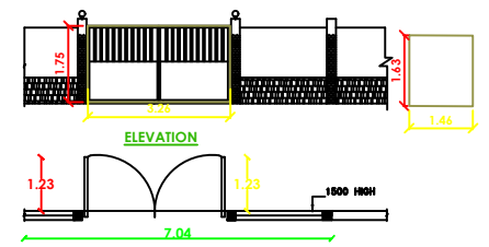
COMPOUND WALL DETAILS
