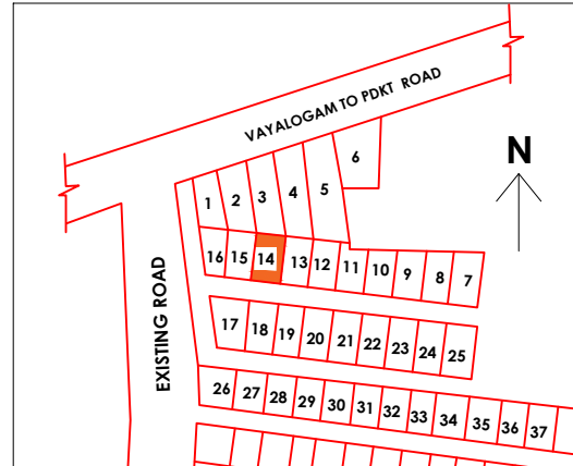
TOPO PLAN
