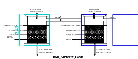
RWH_CAPACITY_L=500
