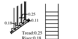
STAIRCASE DETAIL
