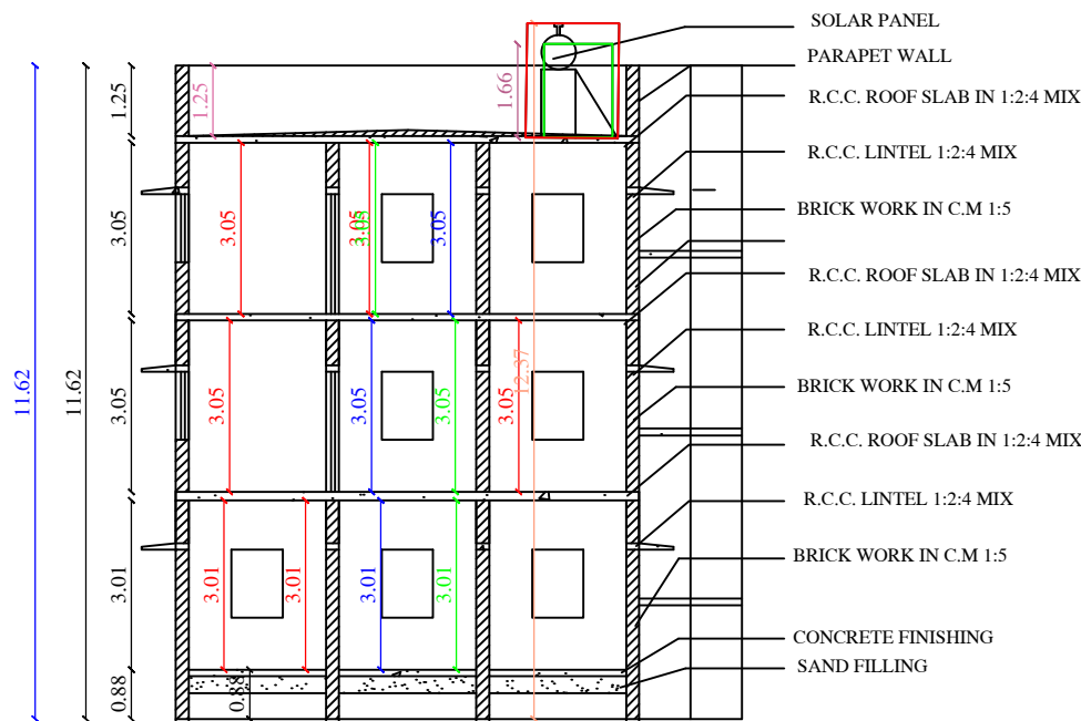
CUT SECTION ON AA
