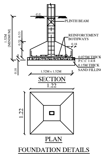
FOUNDATION DETAILS
