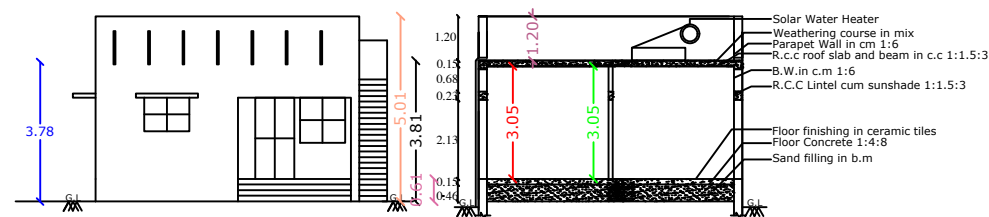
SECTION - "AB "
